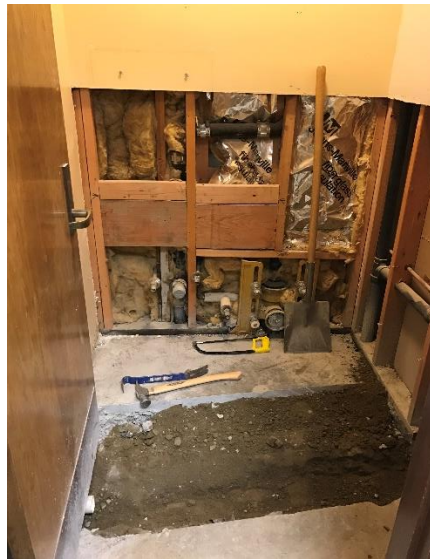
ES NEW PLUMBING AND SANITARY LINES
