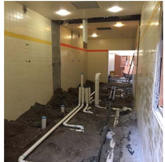
UNDERSLAB WASTE LINE ROUGH-IN AT MS / HS LOCKER ROOMS.
